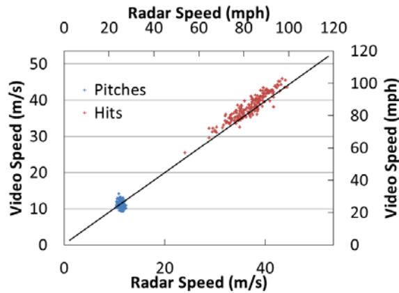
Fig. 3. Comparison of the magnitude of the ball speed between the video and radar tracking systems.
