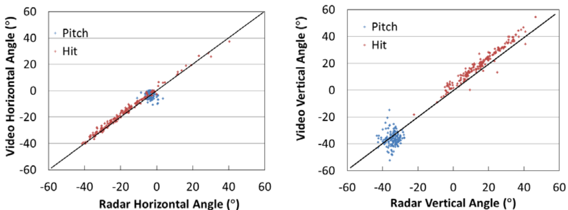
Fig. 2. Comparison of the horizontal and vertical ball trajectory angles between the video and radar. Black lines represent unit slope and ideal correlation.
