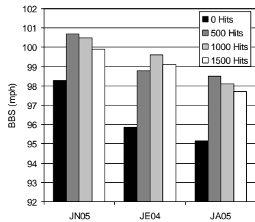
Fig. 4. Change in performance from naturally broken-in bats.
