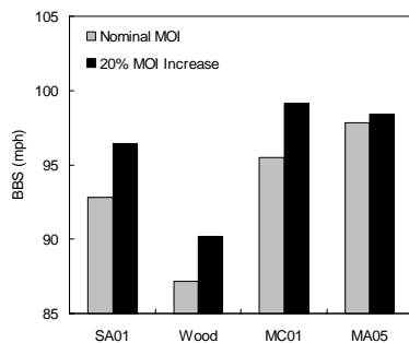
Fig. 2. Comparison of BBS of weighted bats
